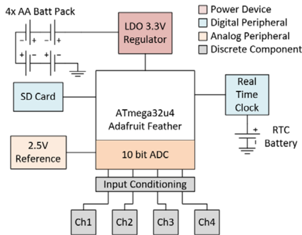
Figure 2: Proposed Architecture
