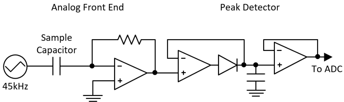
Figure 4: Moisture Sensing Front End
